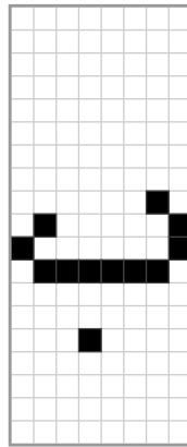
0x1D6
