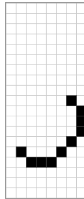
0x1DF
