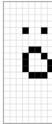
0x1D7
