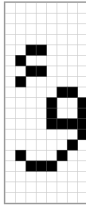
0x1D2
