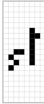
0x1D3
