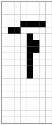
0x1D0
