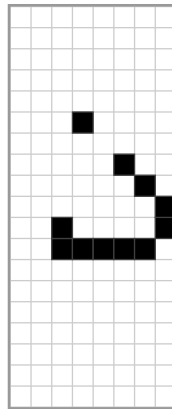
0x1DE
