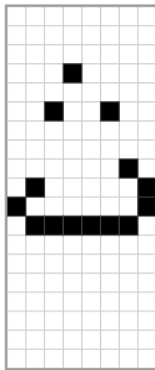
0x1D9
